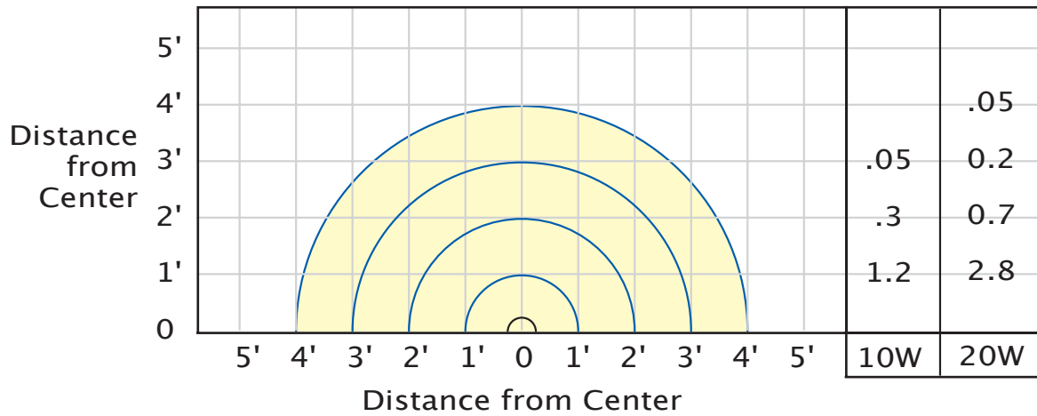
Footcandles at 24" above Grade
